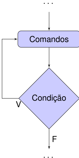
Fluxograma do-while
