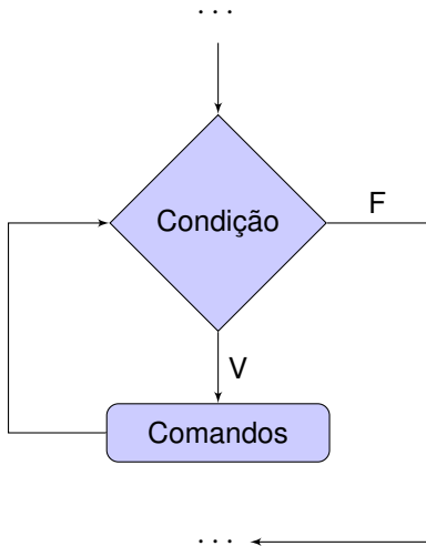
Fluxograma while
